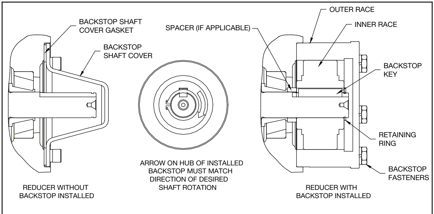
Figure 11 - Backstop Assembly
