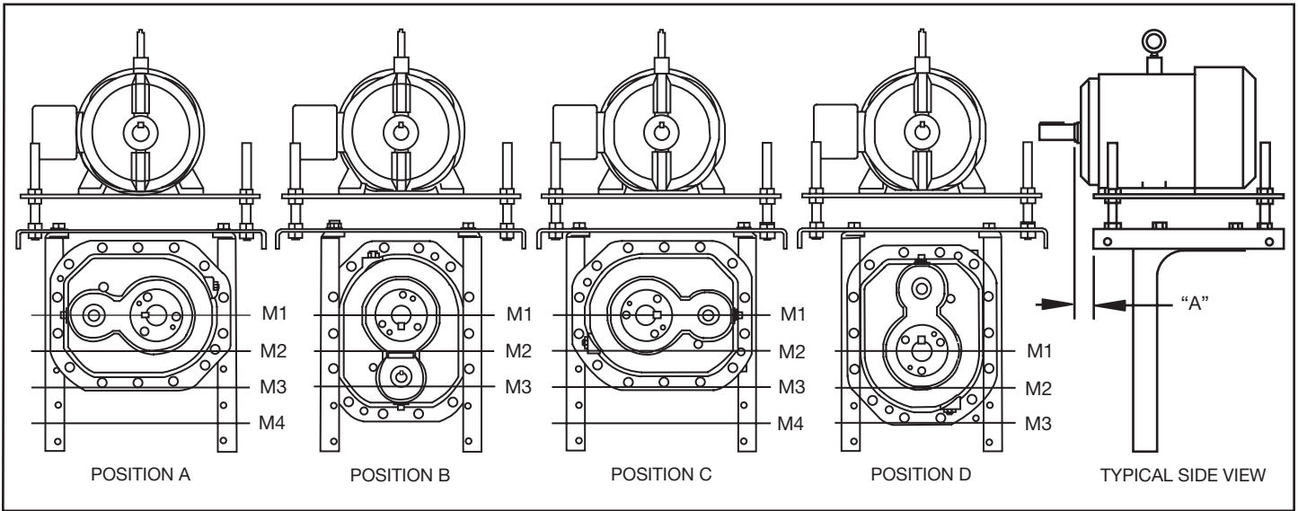
Figure 2 - Mounting Positions
