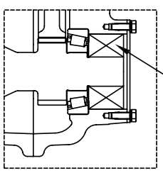
BACKSTOP ASSEMBLY
