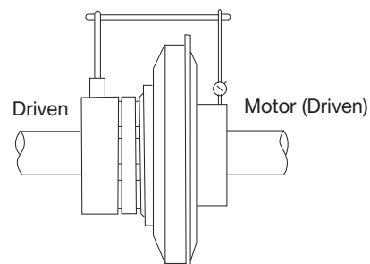
Figure 2 - Parallel Misalignment
