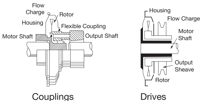
Figure 1 - Housing cross section
