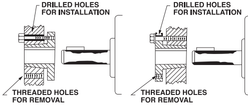
Figure 1 - Conventional Mounting
