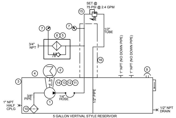
Figure 9 - Hydraulic Schematic
